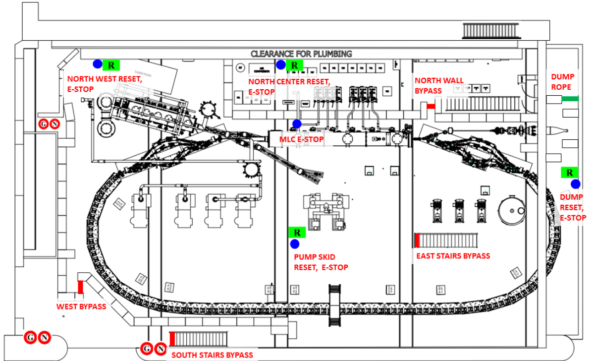
Figure 1: Annotated First Floor Layout as of Nov. 1 st , 2018
