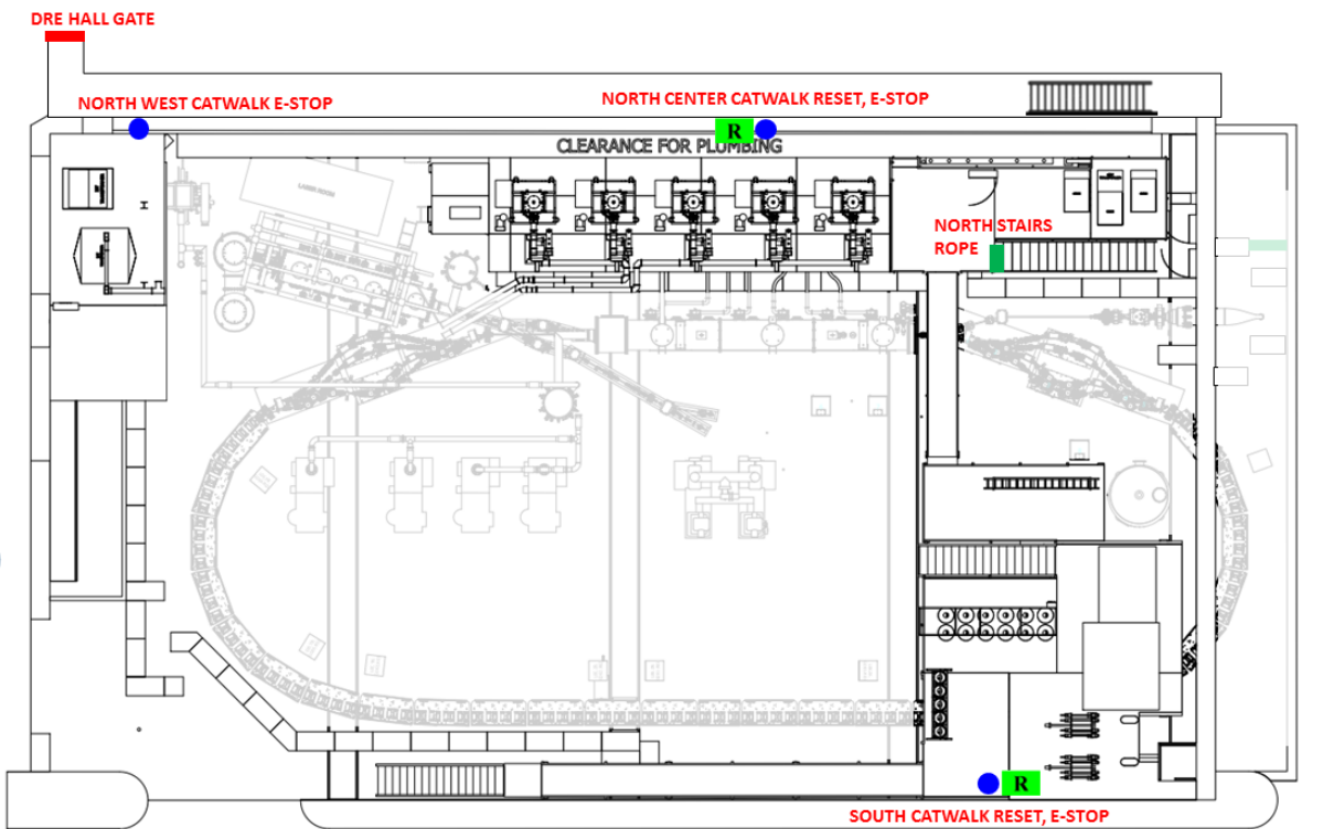
Figure 2: Annotated Second Floor Layout as of Nov. 1 st , 2018
