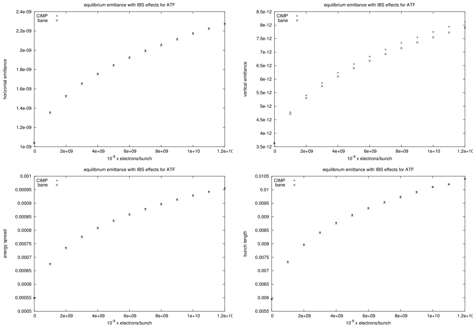
Figure 1: Equilibrium beam parameters for ATF as calculated in BMAD using radiation integrals parameters.
